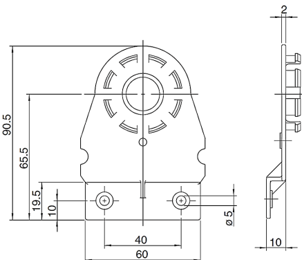
Mounting bracket 6401
