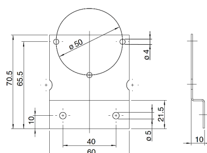
Mounting bracket 6402
