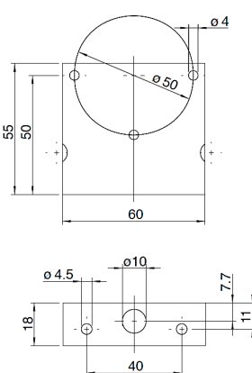
Mounting bracket 6401
