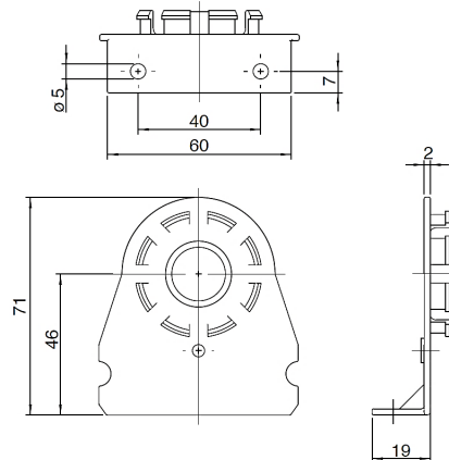
Mounting bracket 648
